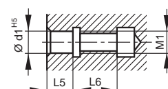
Close-fit hole for type 2 and 3
